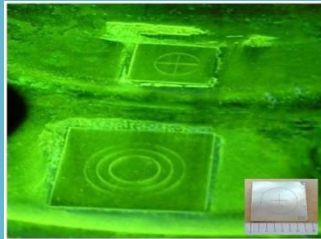
Notched Shim (also called quantitative quality indicator, or QQI)
